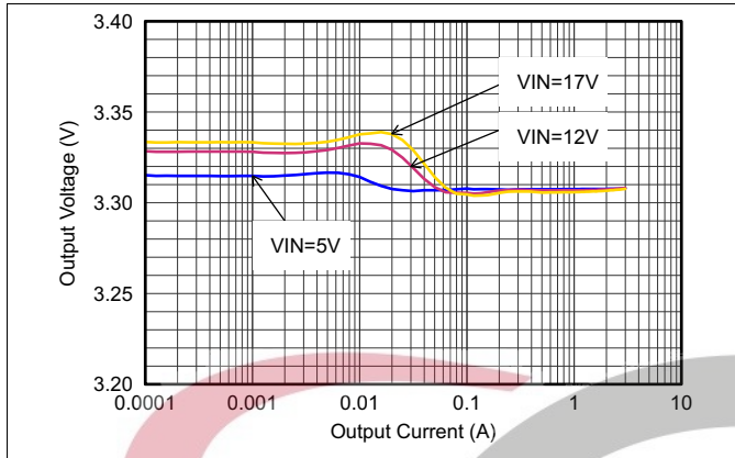
Figure 20. Output Voltage Accuracy (Load Regulation)
