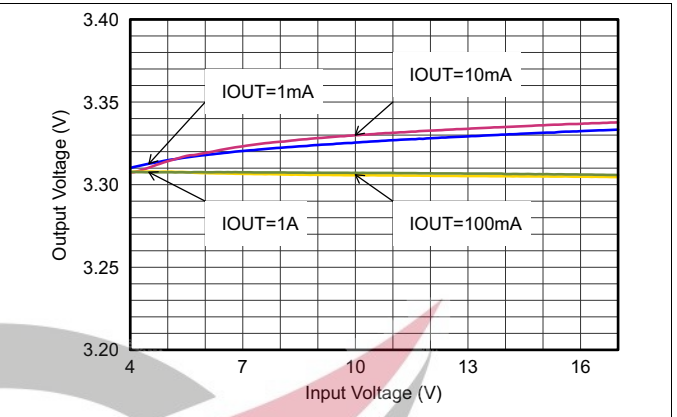
Figure 21. Output Voltage Accuracy (Line Regulation)
