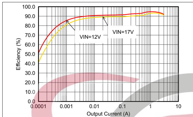
Figure 8. Efficiency With 1.25 MHz, Vout = 5 V
